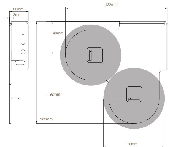
RB09-8384-xxx122 | Easy-Lock Combo - Idle End
