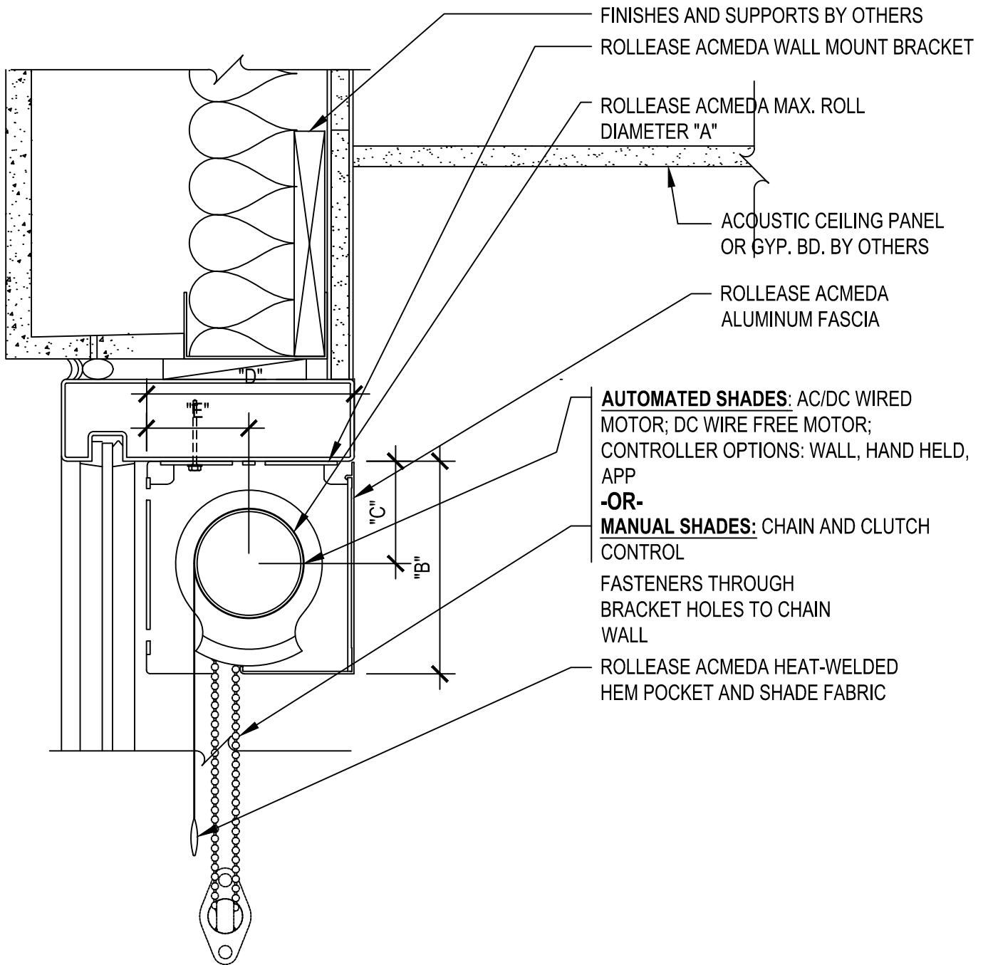
"SINGLE RS 38 (SKYLINE SERIES) WITH FASCIA" DIMENSION TABLE
