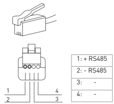
Data Cable: RJ9
