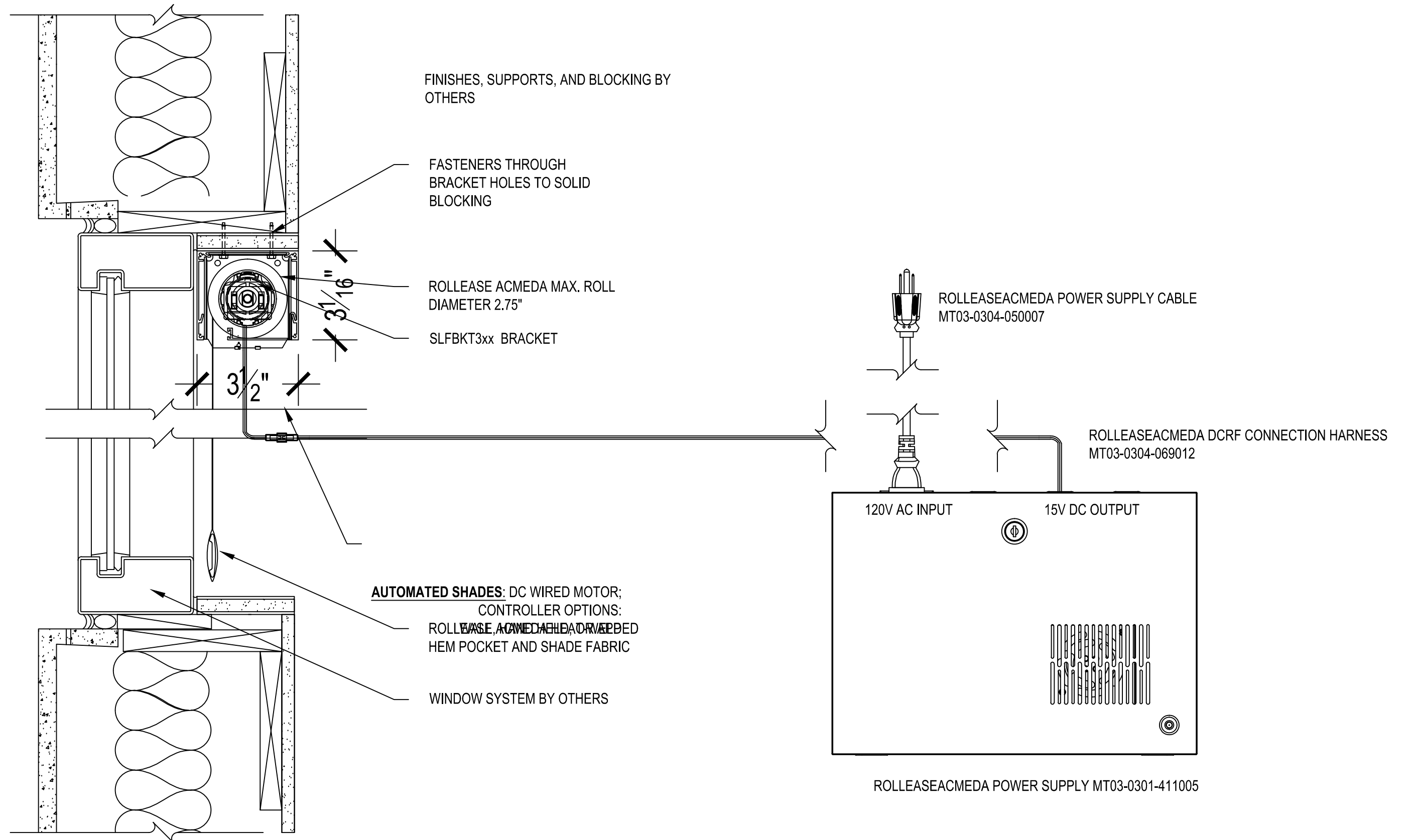
CS1 3 IN POCKET SINGLE - PUNCH WINDOW SCALE: 3"=1'-0" LOW VOLTAGE MOTOR HEADER MOUNT
